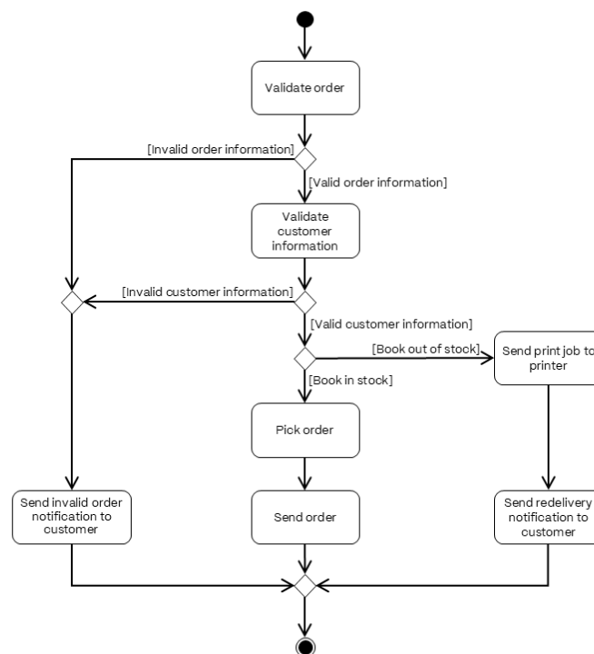
Figure 3.11 Example of a UML activity diagram
