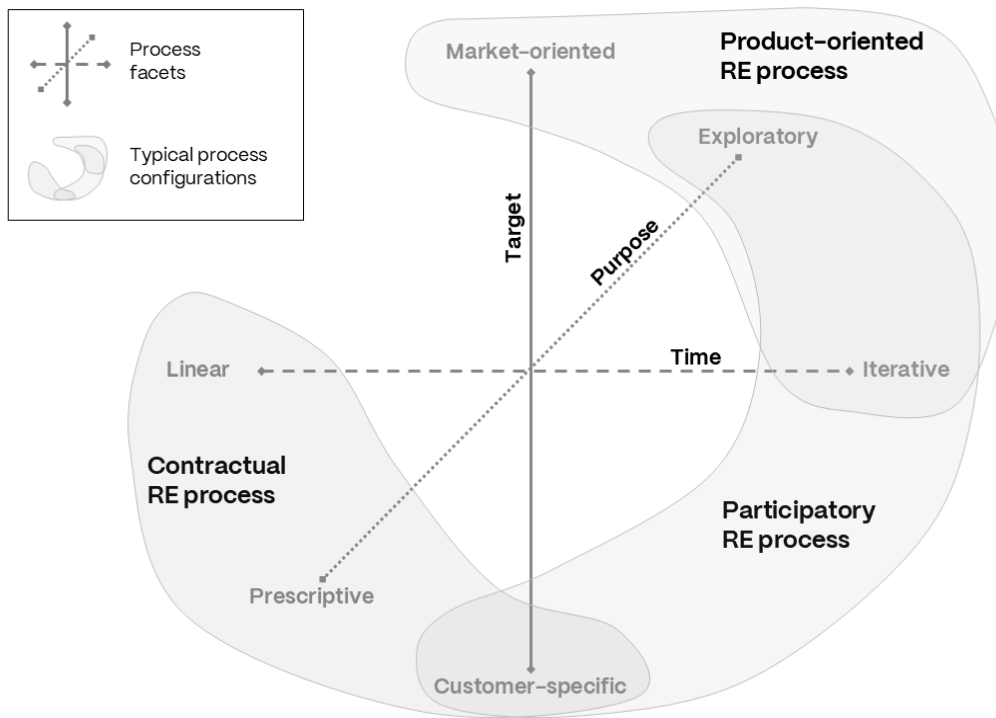
Figure 5.2 Three typical RE process configurations and their relationship to the three facets
