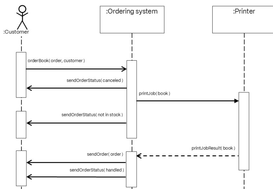
Figure 3.17 Example of a UML sequence diagram
