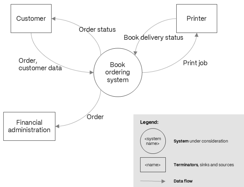
Figure 3.5 Example of a context diagram using a DFD
