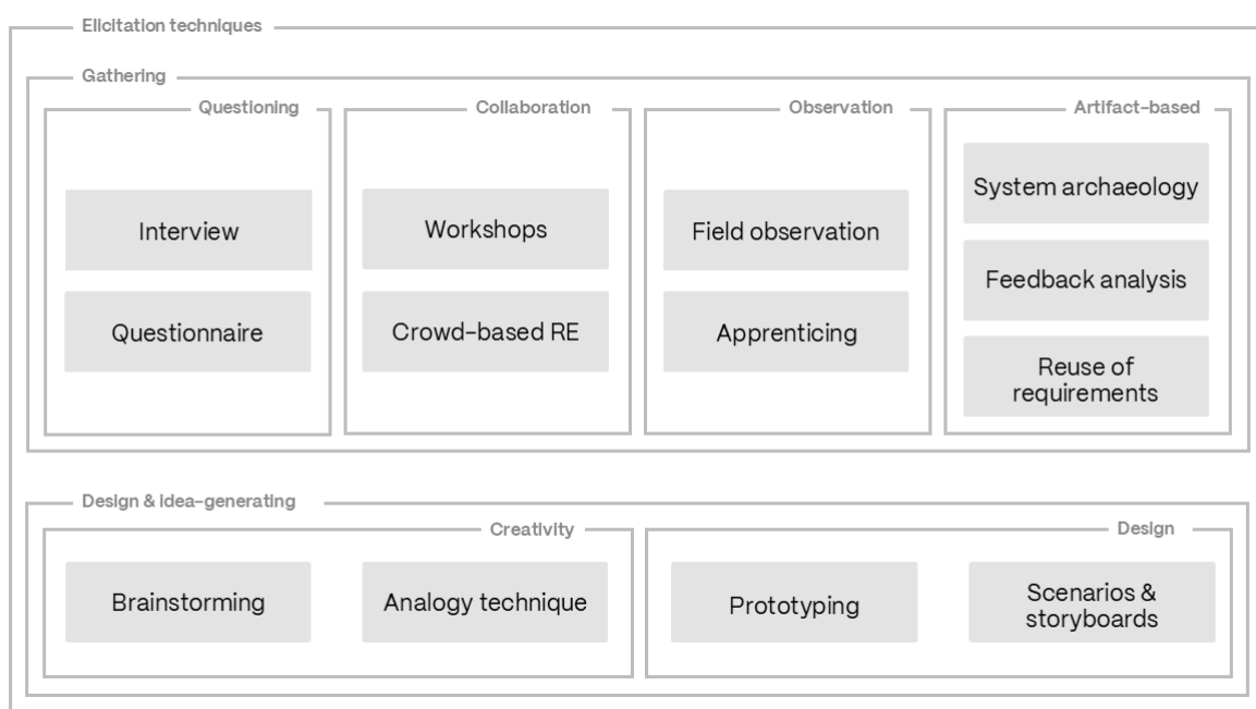
Figure 4.4 An overview of elicitation techniques
